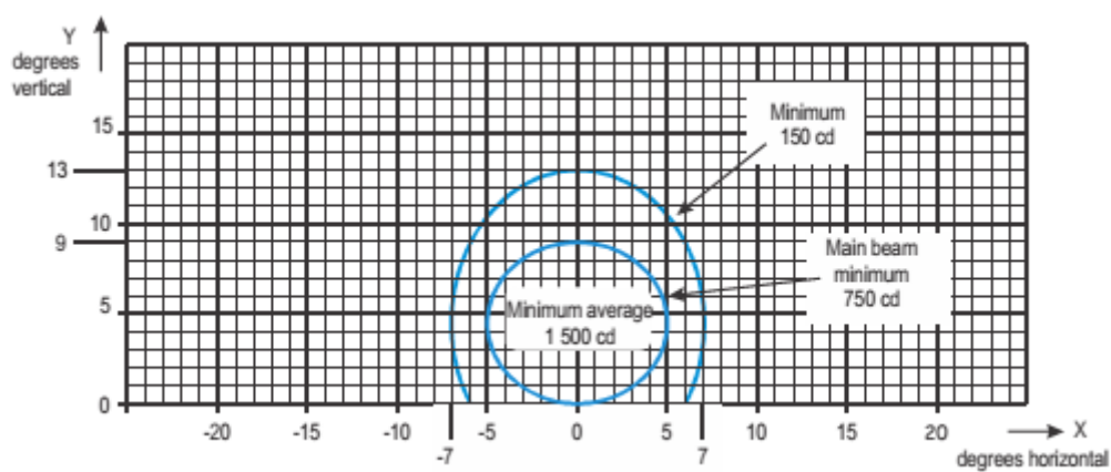
Figure A2-26. Isocandela diagram for take-off and hold lights (THL) (red light)
