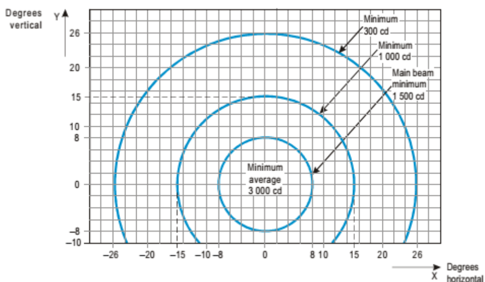
Figure A2-25. Isocandela diagram for each light in high-intensity runway guard lights, Configuration A
