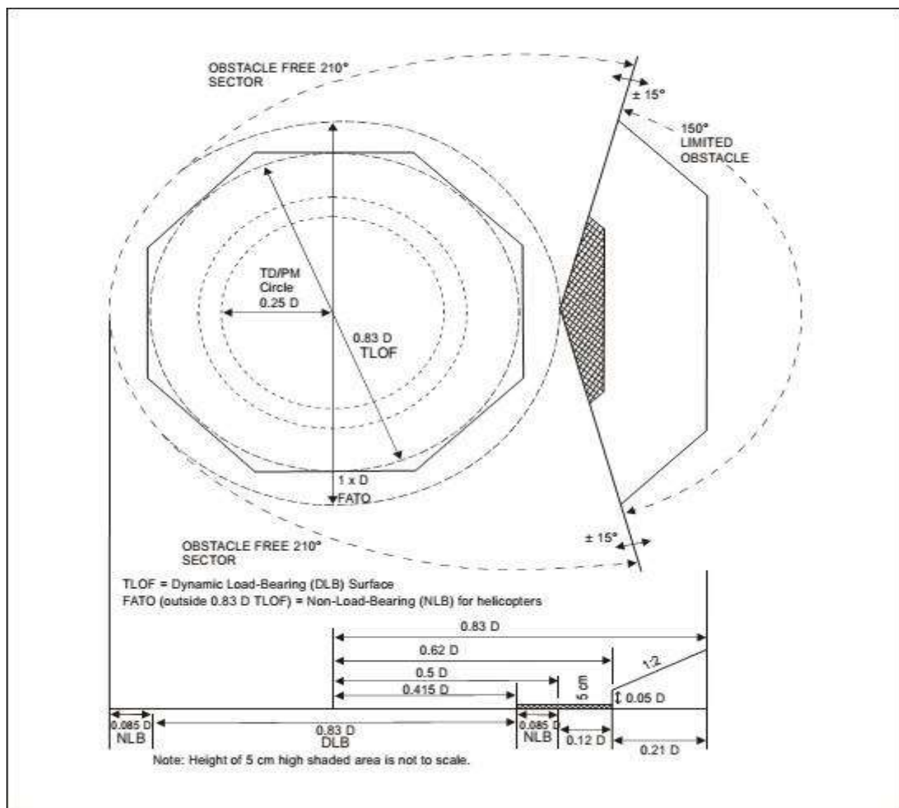
Figure 4-9. Helideck obstacle limitation sectors and surfaces for a TLOF of 0.83 D and larger
