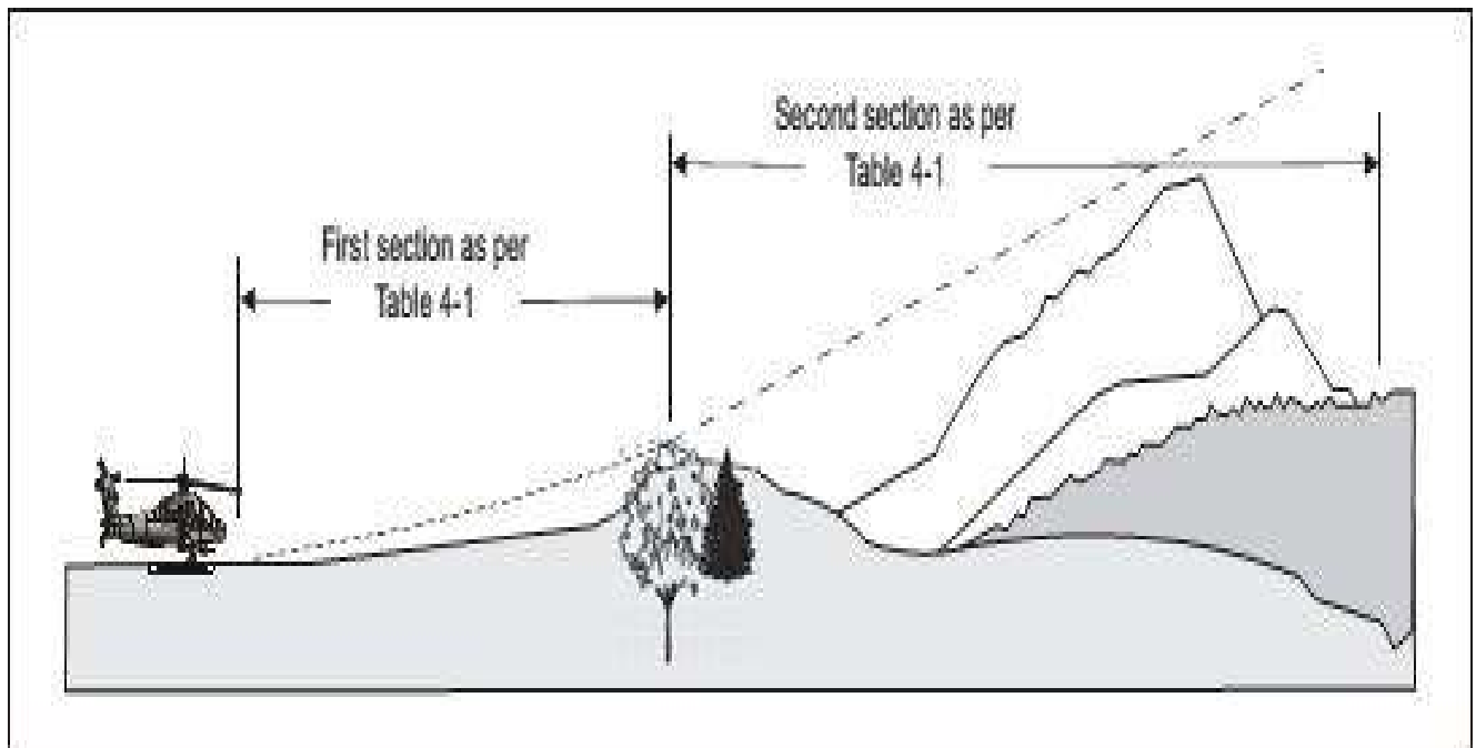
b) Approach and take-off climb surfaces - “B” slope profile - 8% and 16% design
