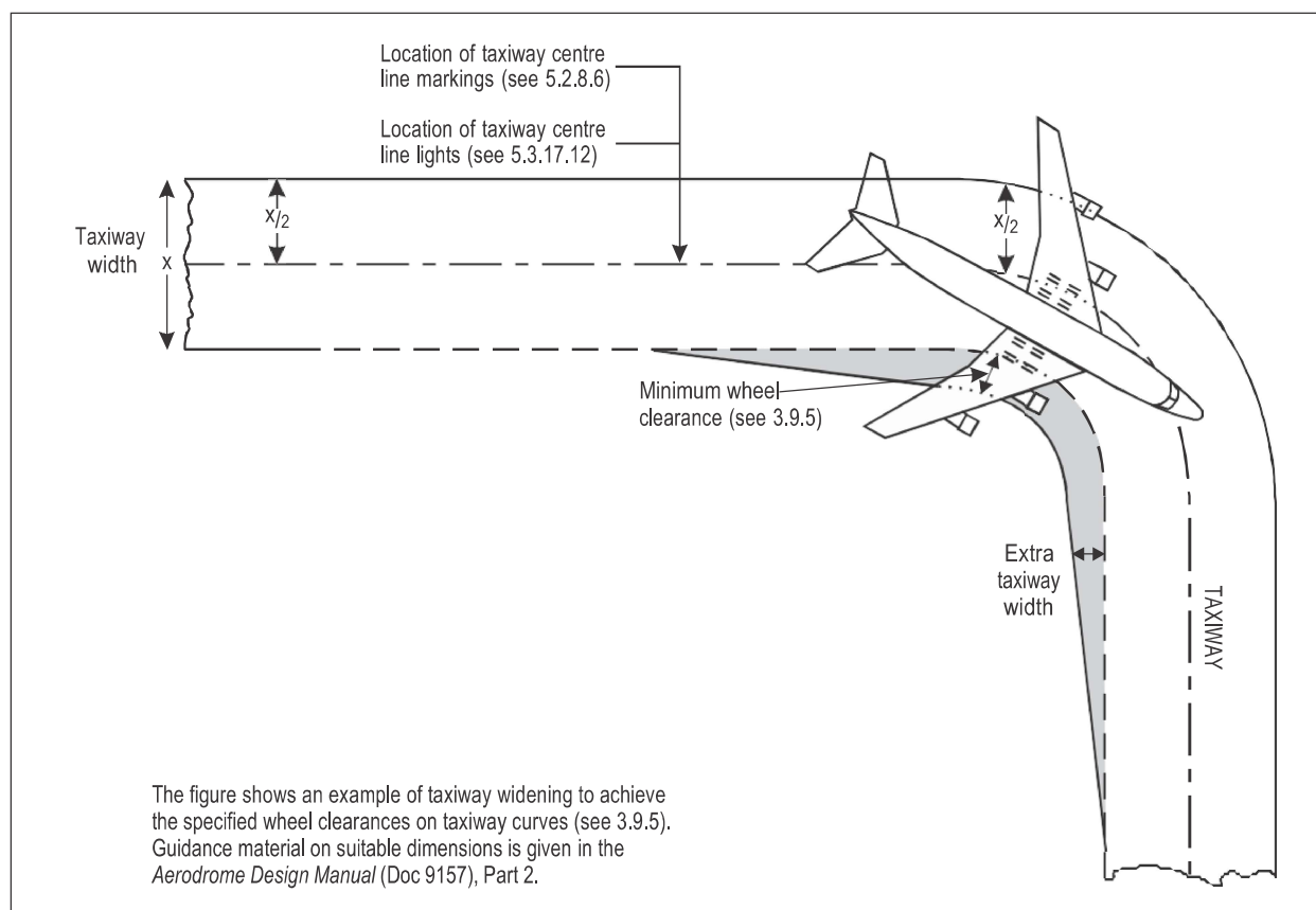
Figure 10. 2: Taxiway curve
