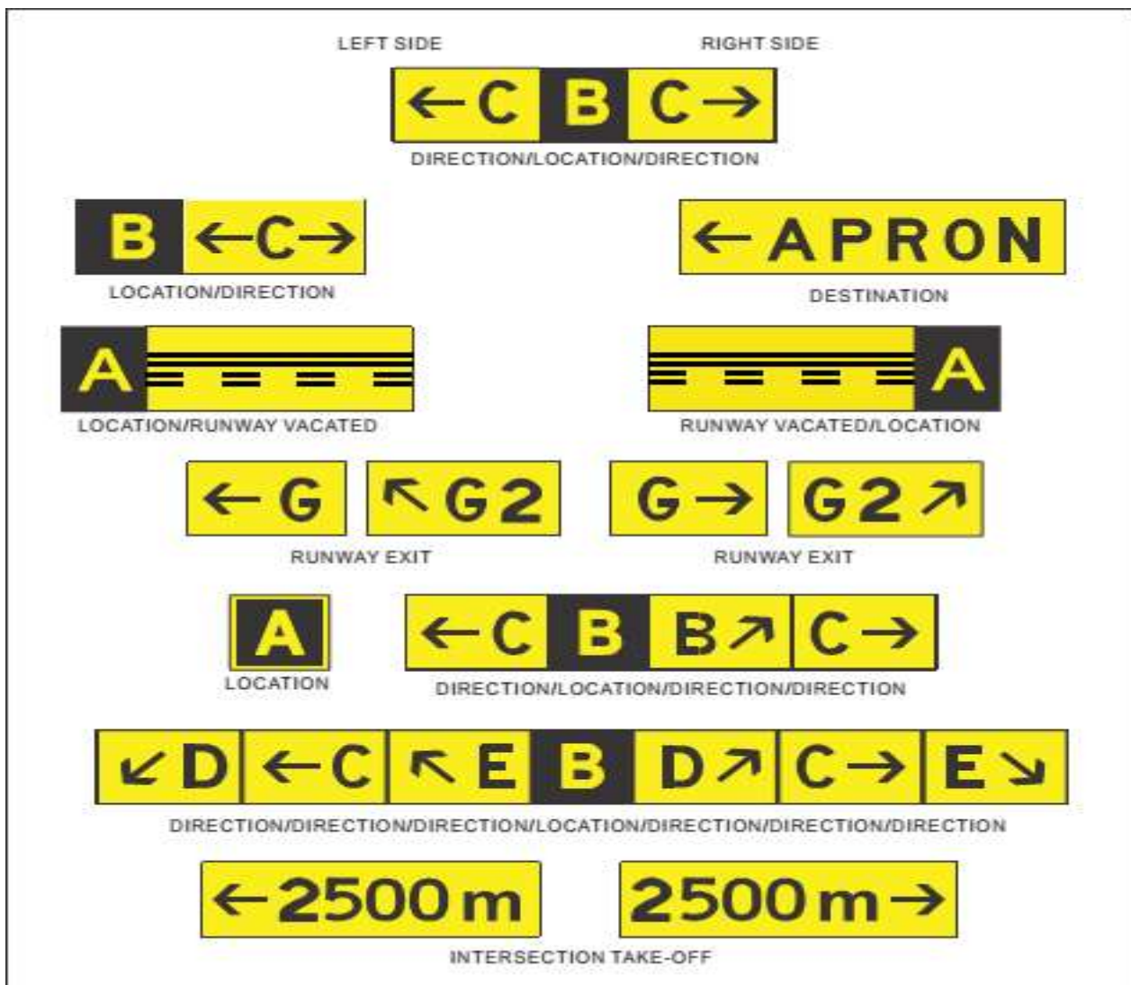
Figure 12. 38: Information signs
