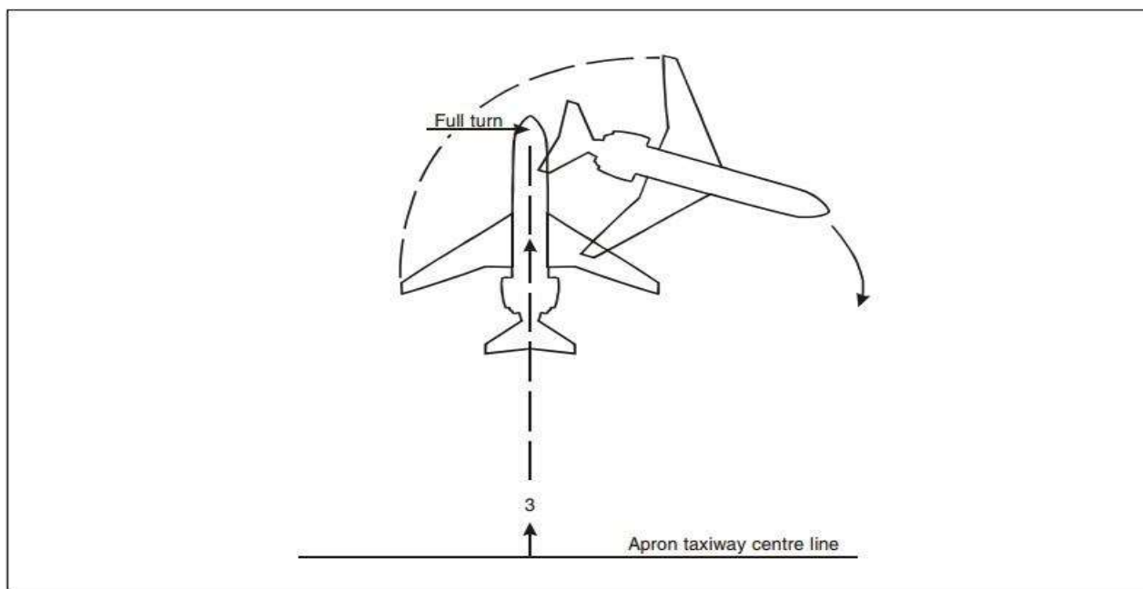
Figure 12. 12: Straight lead-in line
