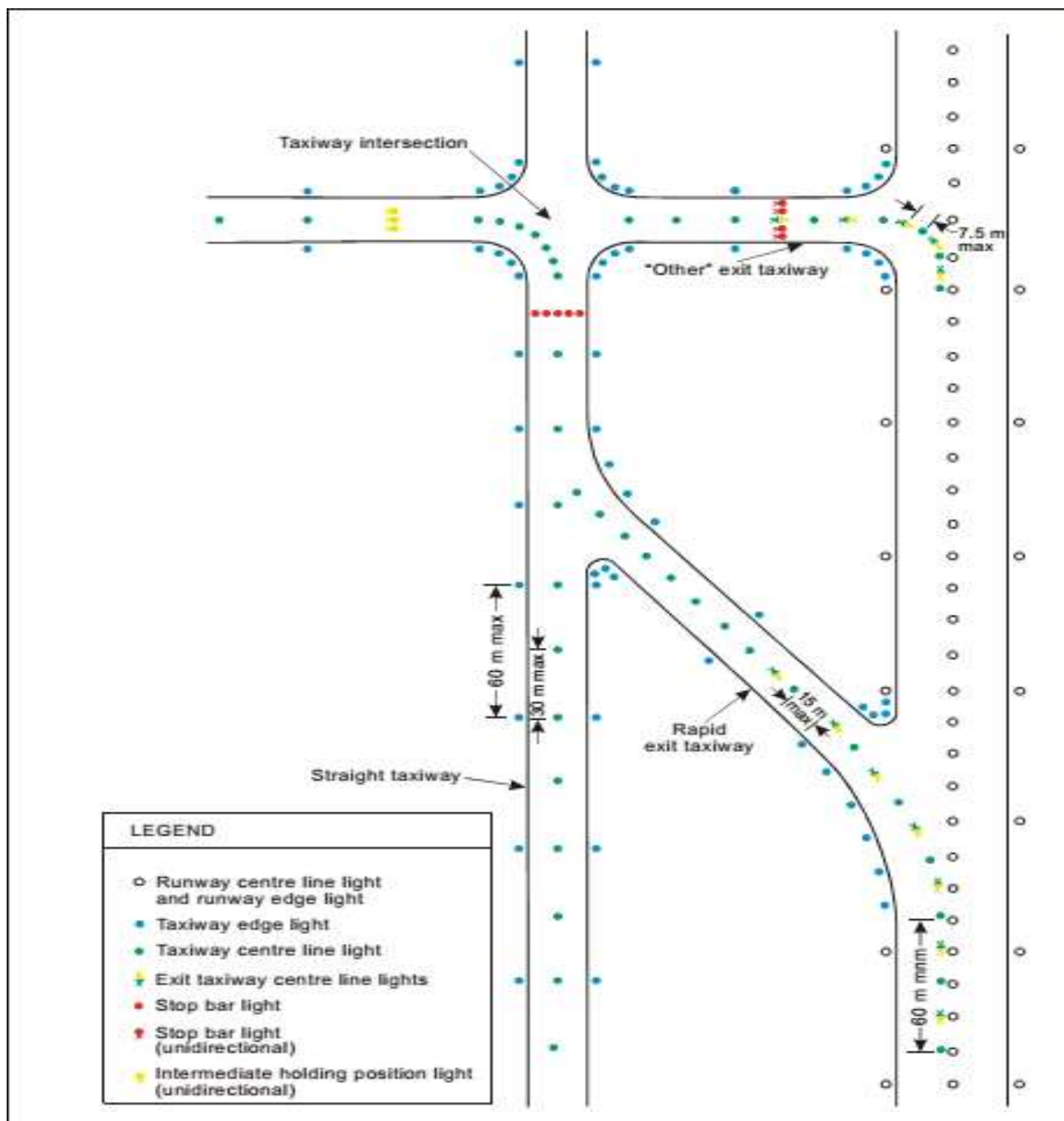
Figure 12. 34: Taxiway lighting
