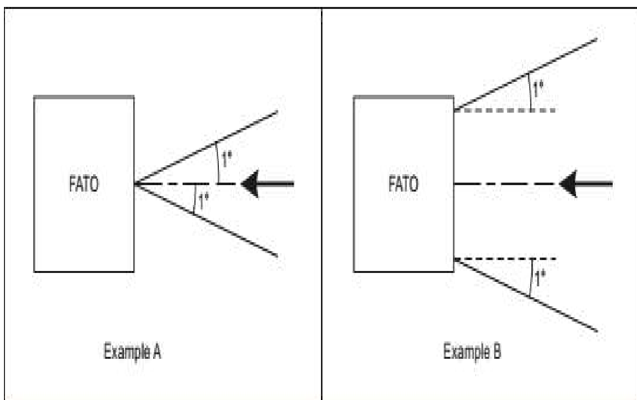
Figure 5-13. Divergence of the “on track” sector
