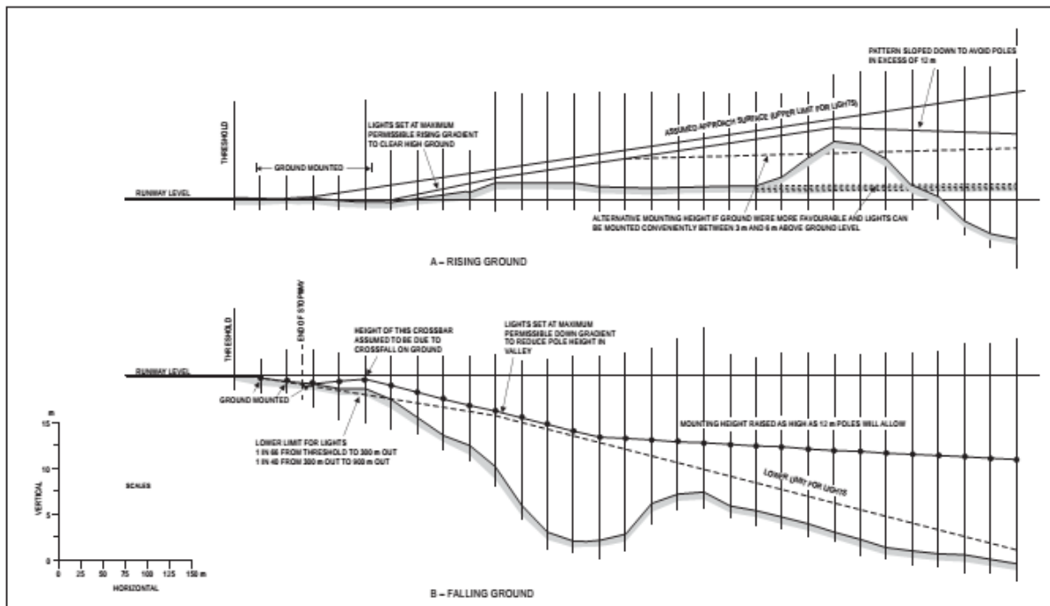
Figure A-9. Vertical installation tolerance
