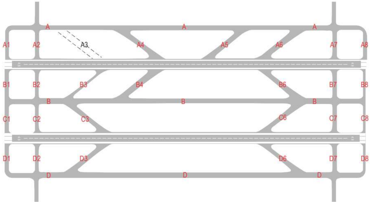
Figure 1-5. Suggested nomenclature for complex taxiway system
