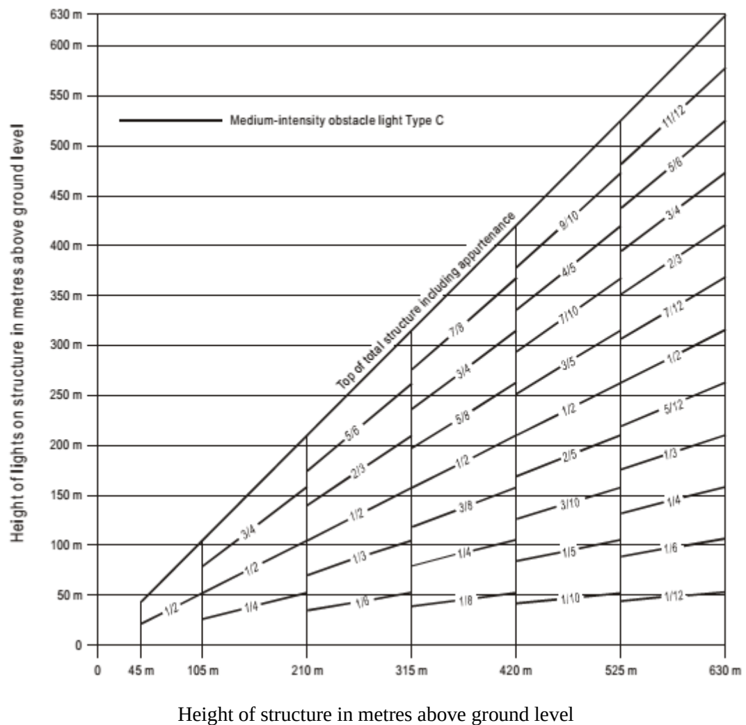
Figure A6-3. Medium-intensity fixed-red obstacle lighting system, Type C
