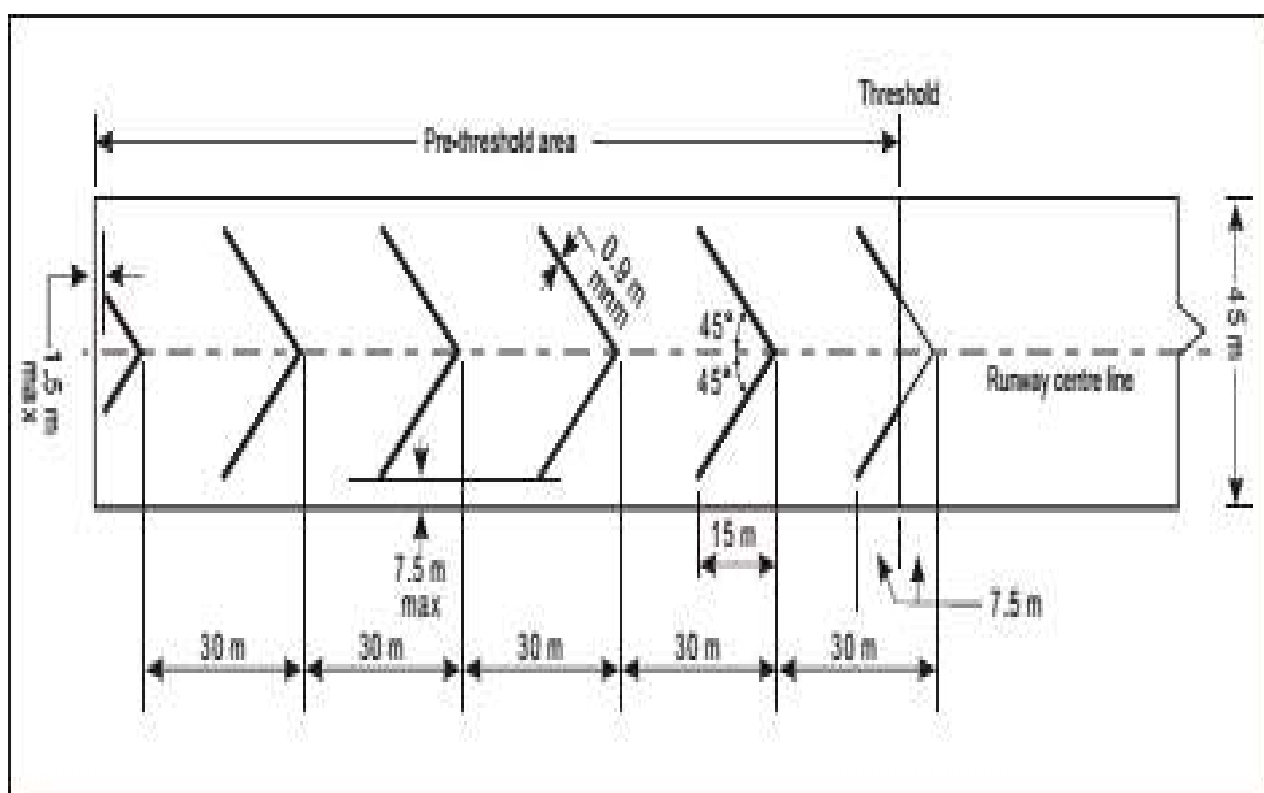
Figure 14. 3: Pre-threshold marking
