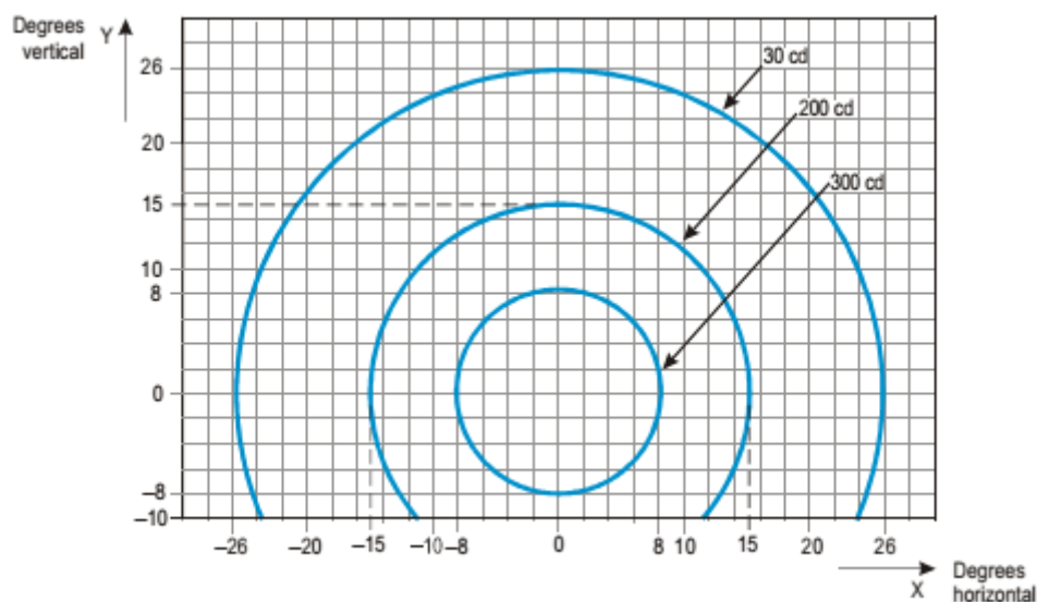
Figure A2-24. Isocandela diagram for each light in low-intensity runway guard lights, Configuration A
