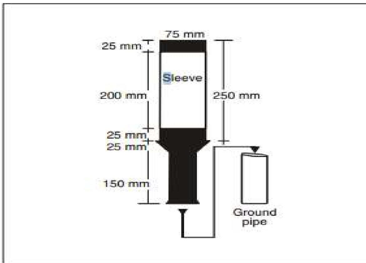
Figure 12. 42: Taxiway edge marker
