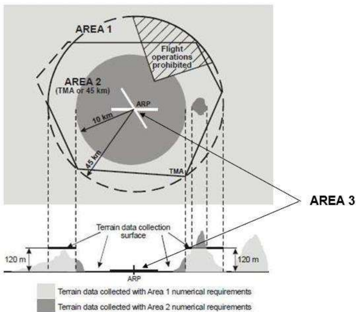
Figure 9. 1: Terrain and obstacle coverage areas
