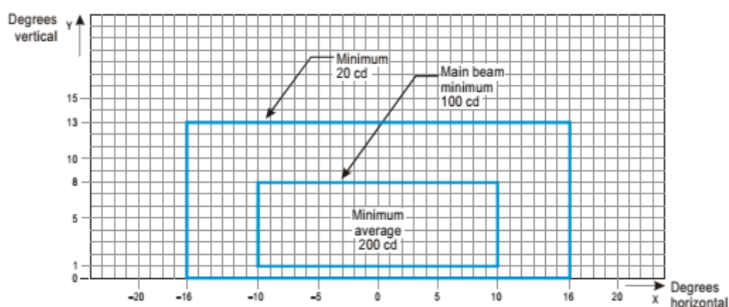
Figure A2-12. Isocandela diagram for taxiway centre line (15 m spacing), RELs, no-entry bar and stop bar lights in straight sections intended for use in runway visual range conditions of less than a value of 350 m where large offsets can occur and for low-intensity runway guard lights, Configuration B
