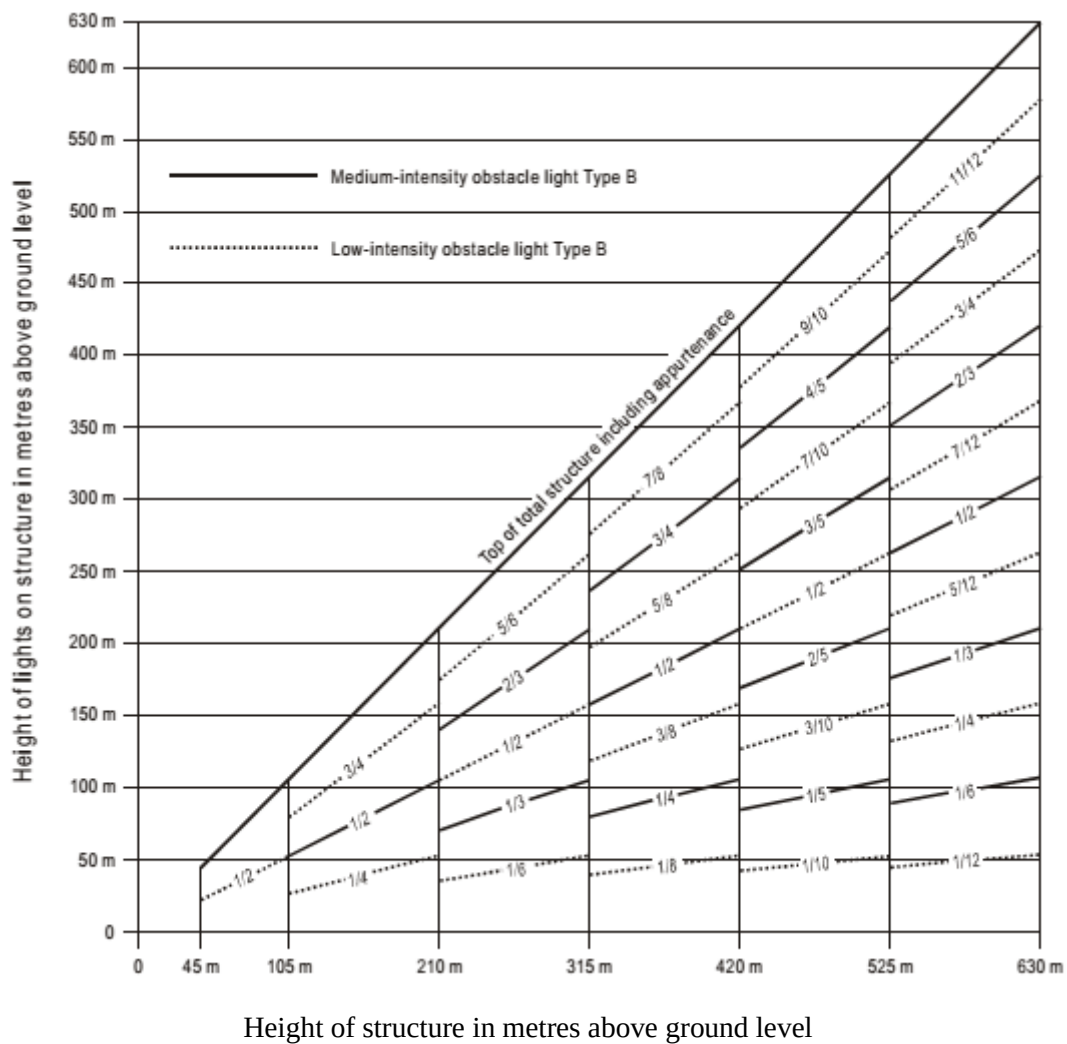
Figure A5-2. Medium-intensity flashing-red obstacle lighting system, Type B
