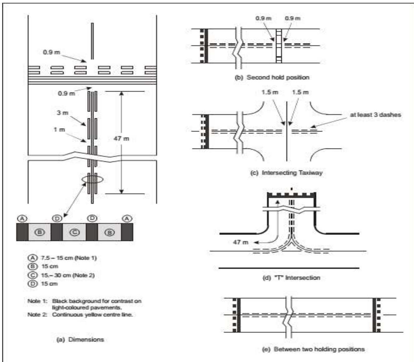
Figure 12. 7: Enhanced taxiway centre line marking
