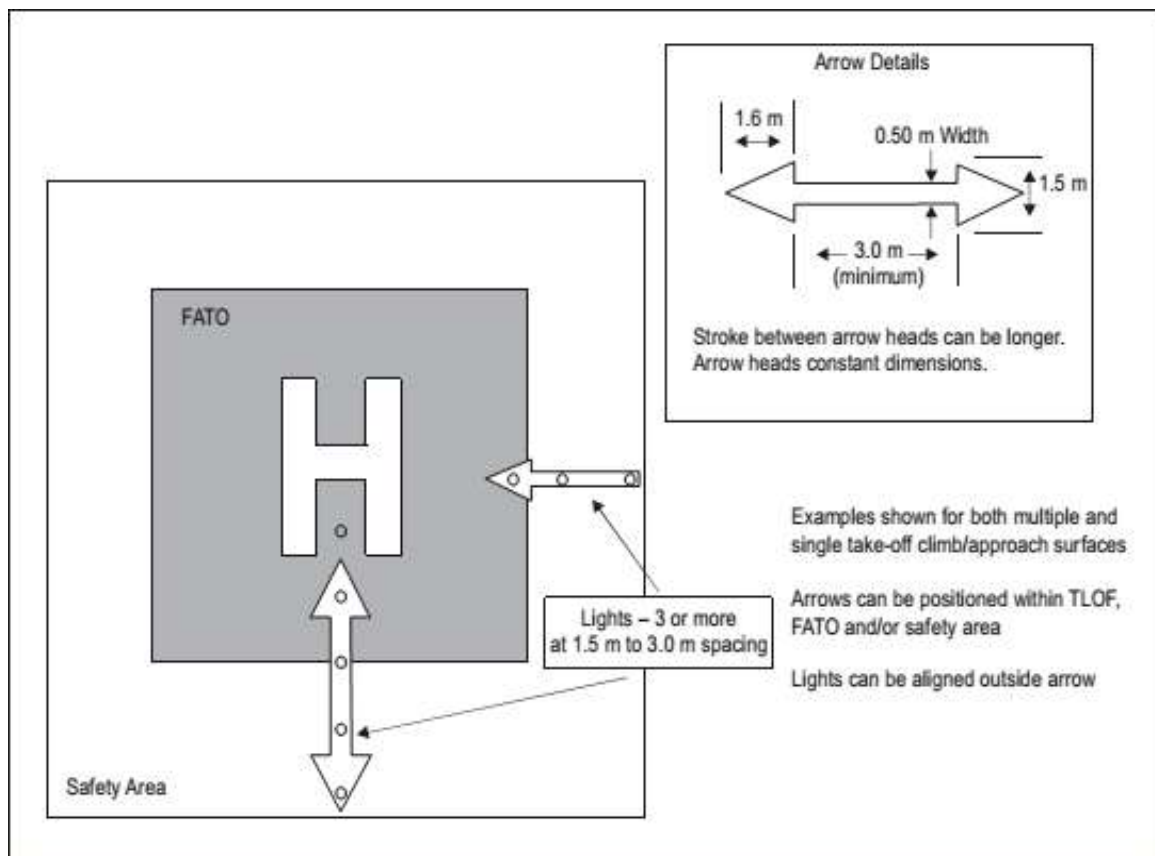
Figure 5-9. Flight path alignment guidance markings and lights
