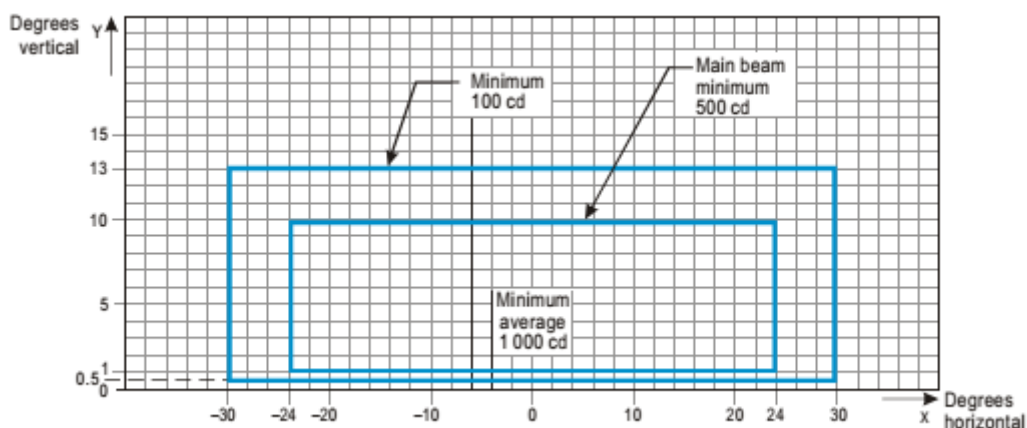
Figure A2-20. Isocandela diagram for high-intensity runway guard lights, Configuration B
