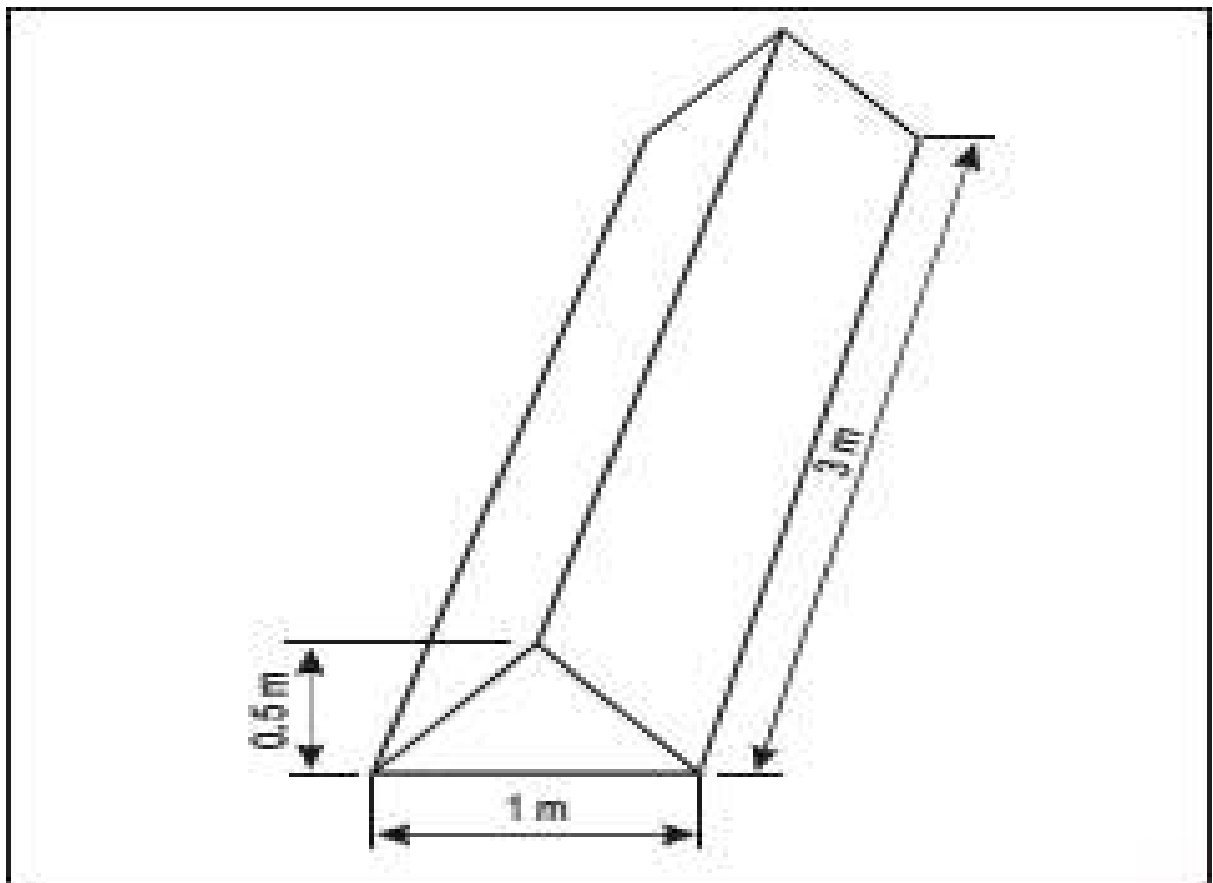
Figure 12. 43: Boundary markers
